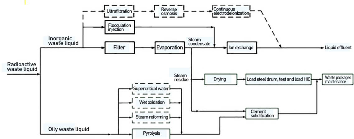
Figure 3. The technical route of radioactive waste liquid treatment in China
